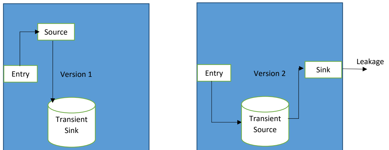
Figure 3: Attack Model
